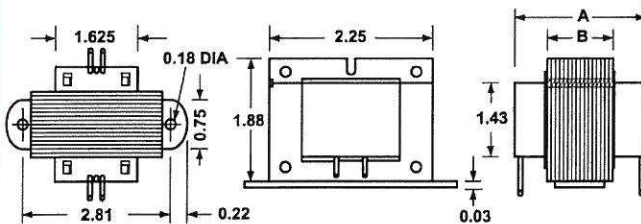
Type HX - Foot Mount
