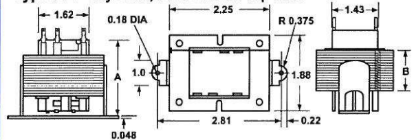
Type AB - Foot Mount, Pri & Sec on Opposite Side
