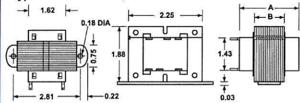
Type AE - Laydown, Pri & Sec on Top Side
