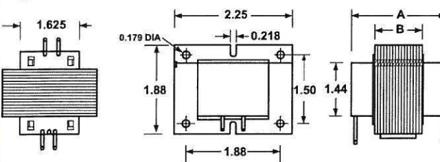
Type GX - Panel Mount
