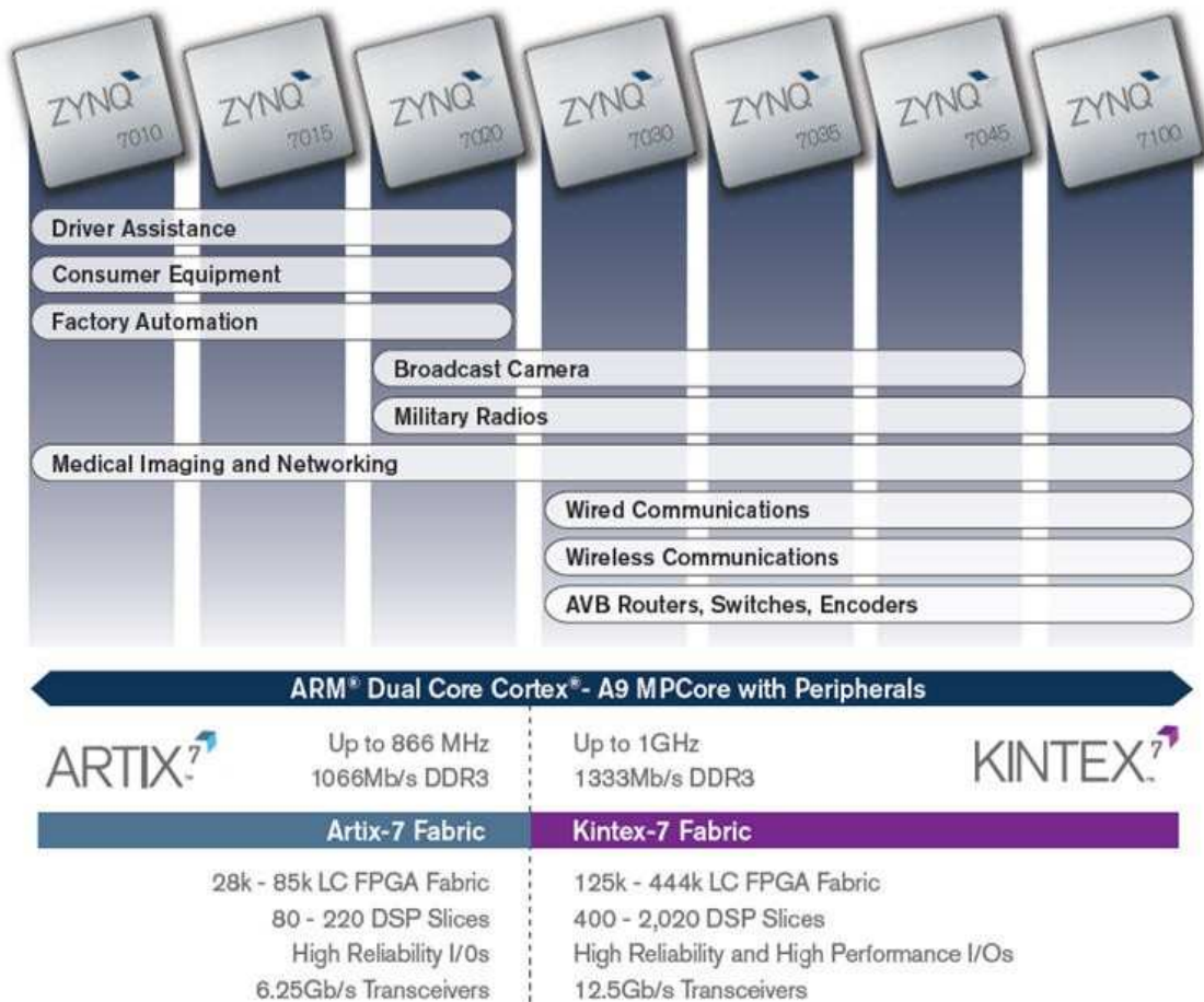
Figure 1-2 ZYNQ-7000 Device Family
