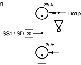
Figure 8 - 3uA current source for discharging soft start-capacitor during Hiccup mode
