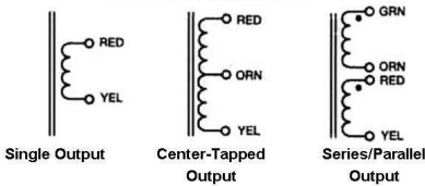
Secondary Schematics
