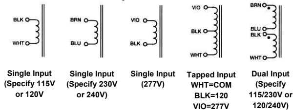
Primary Schematics
