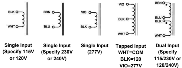
Primary Schematics
