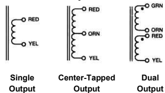
Secondary Schematics
