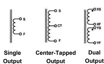
Secondary Schematics
