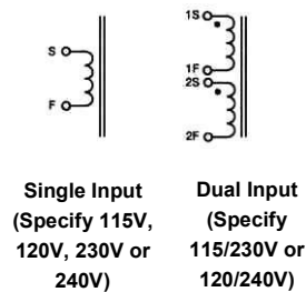
Primary Schematics
