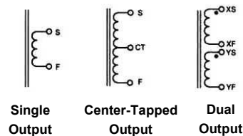
Secondary Schematics
