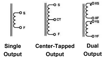
Secondary Schematics
