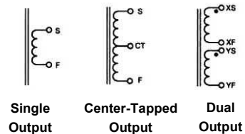
Secondary Schematics
