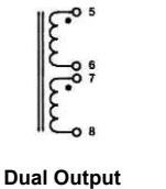
Secondary Schematics
