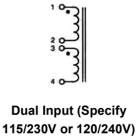
Primary Schematics
