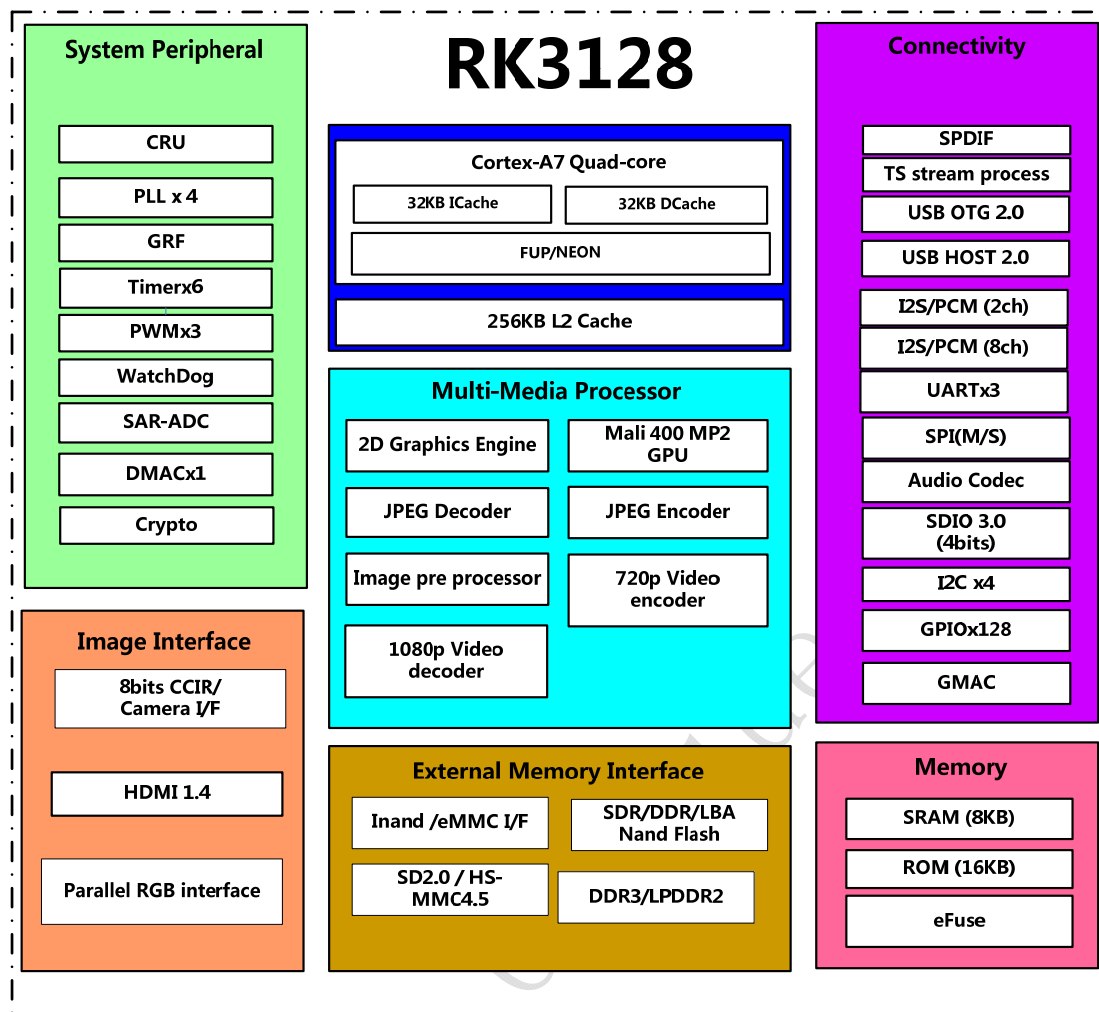
Fig.1-1RK3128 Block Diagram
