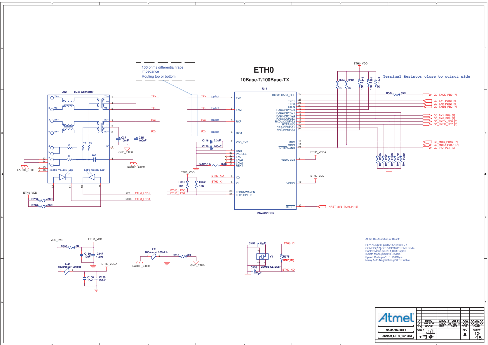
Figure 4-60. Ethernet_ETH0_10/100M
