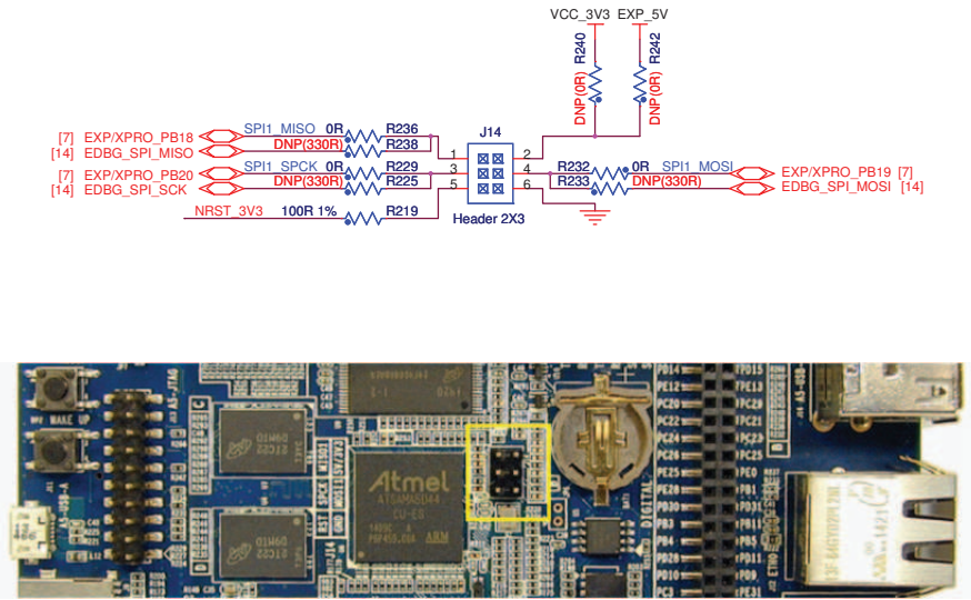
Figure 4-29. J14 Connector
