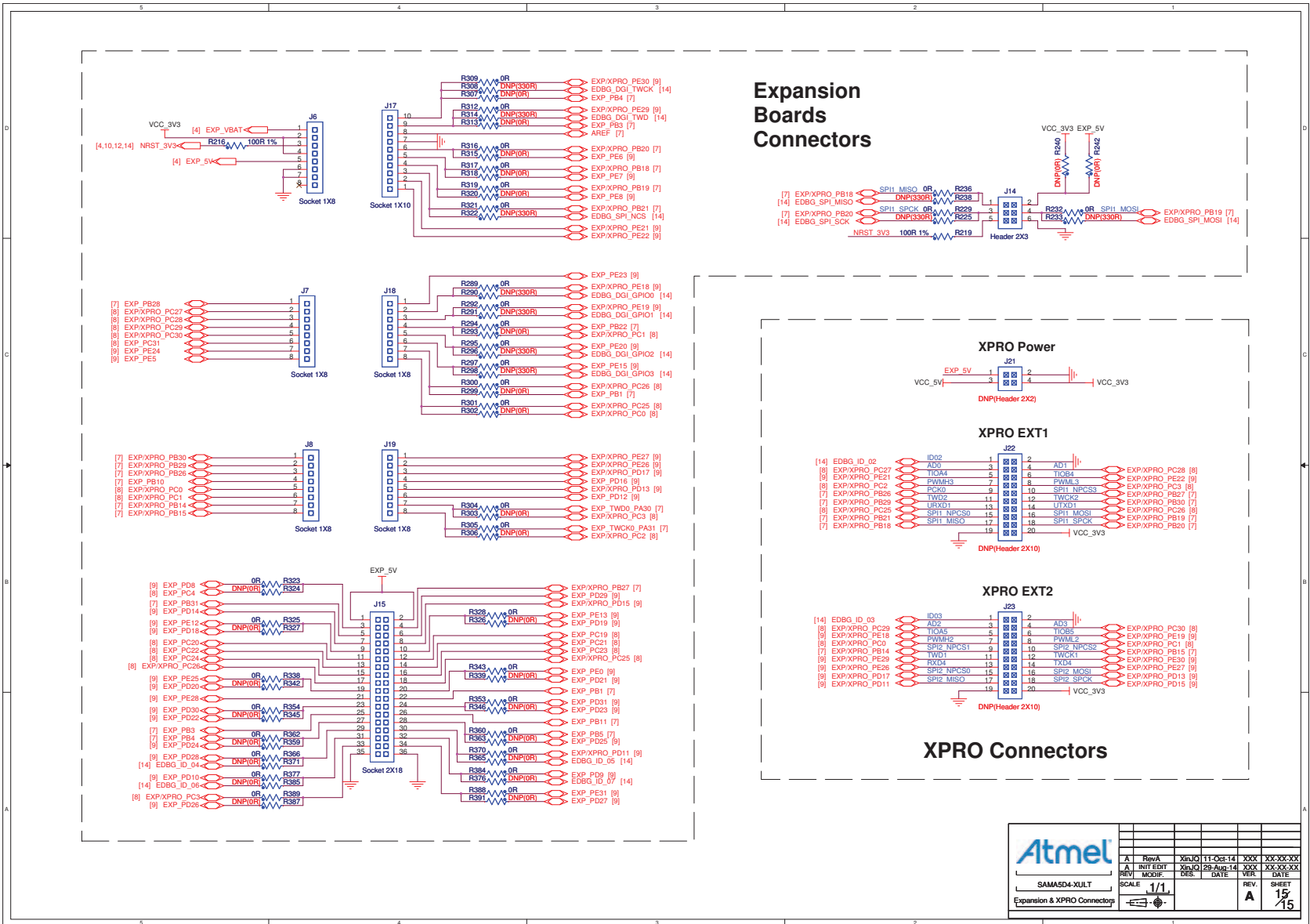
Figure 4-63. Expansion and XPRO Connectors
