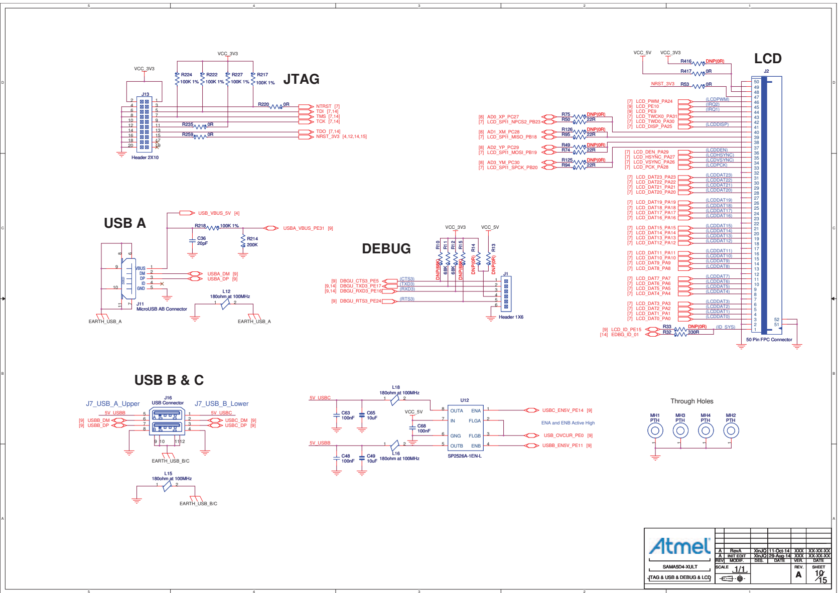
Figure 4-58. JTAG, USB, DEBUG, and LCD
