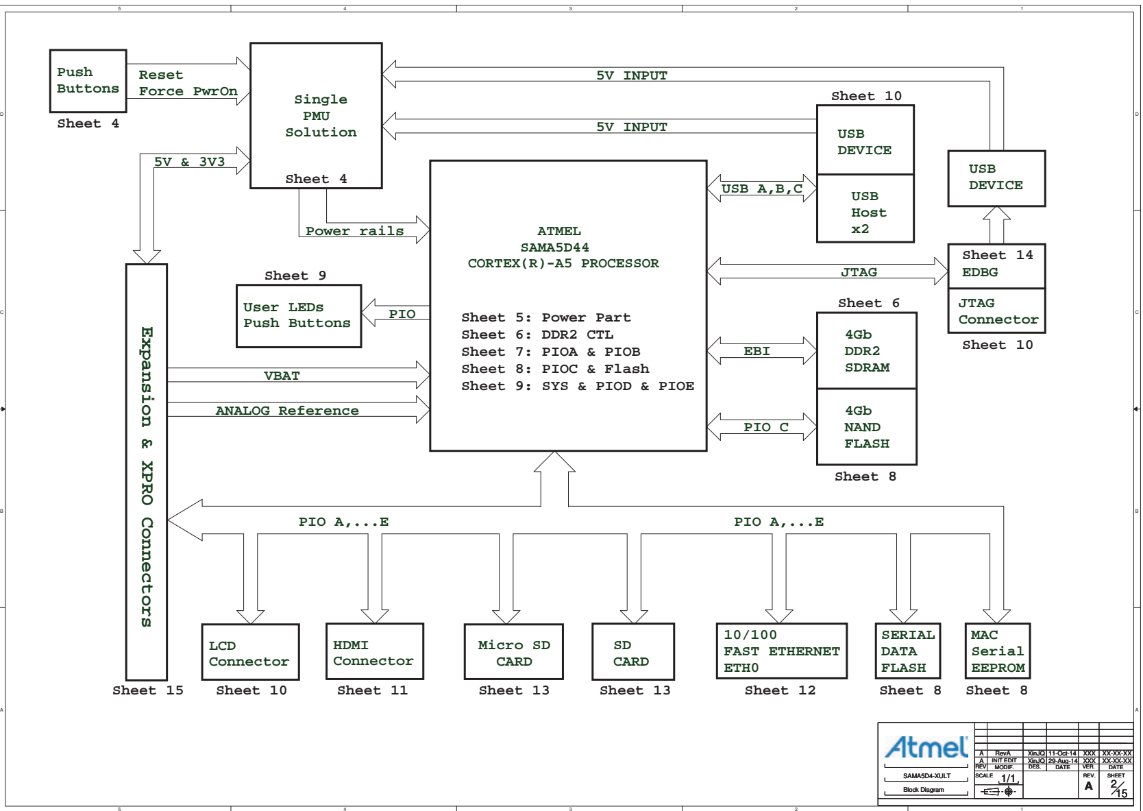
Figure 4-50. Block diagram
