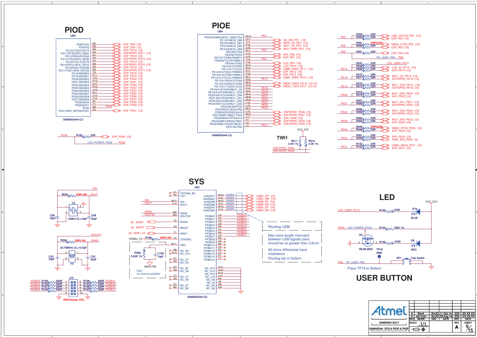
Figure 4-57. SAMA5D4 - SYS, PIOD, and PIOE
