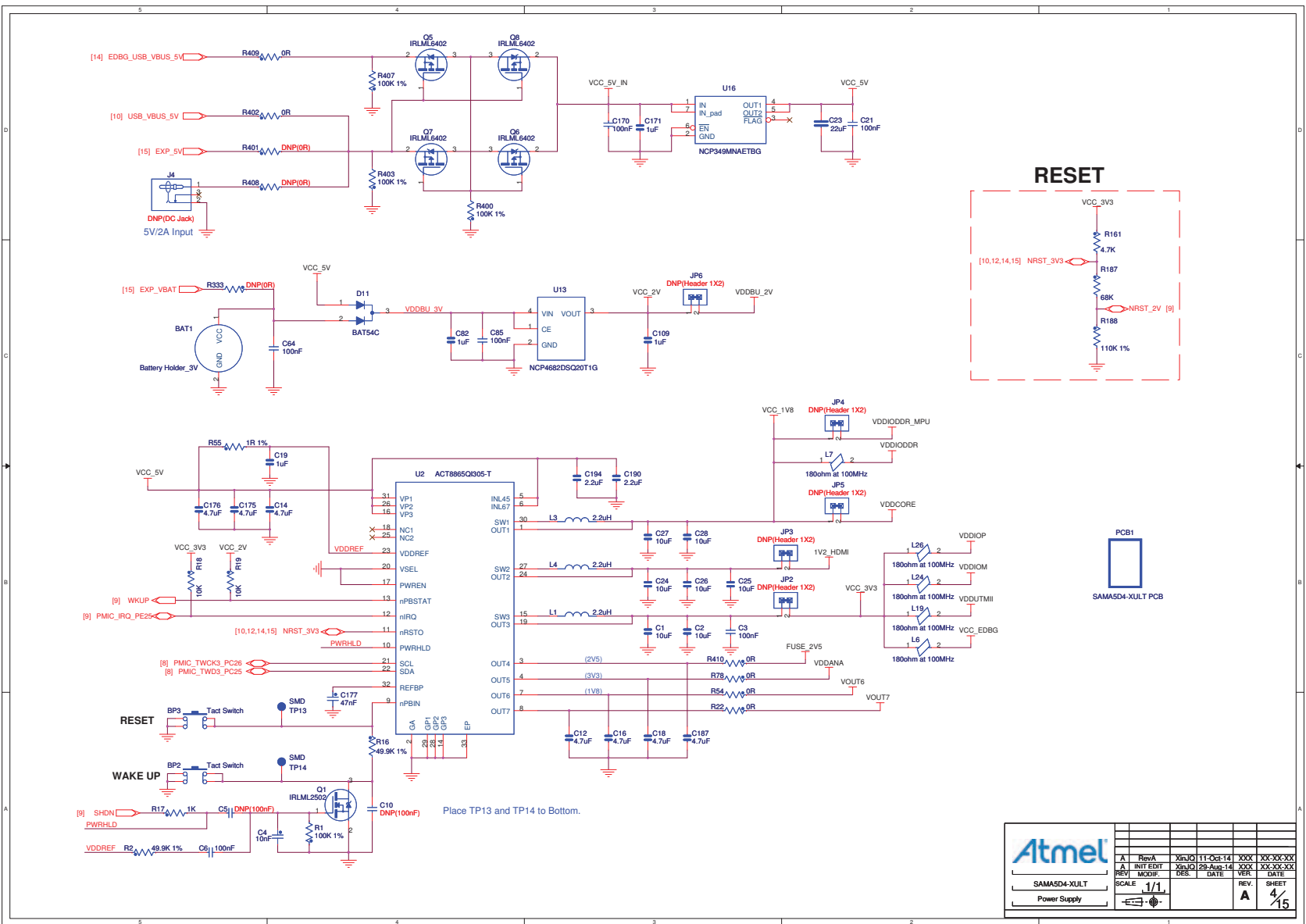
Figure 4-52. Power Supply
