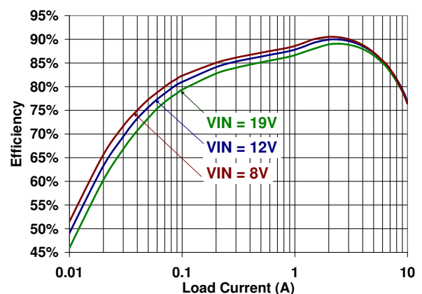
Figure 2: IR3475 Efficiency
