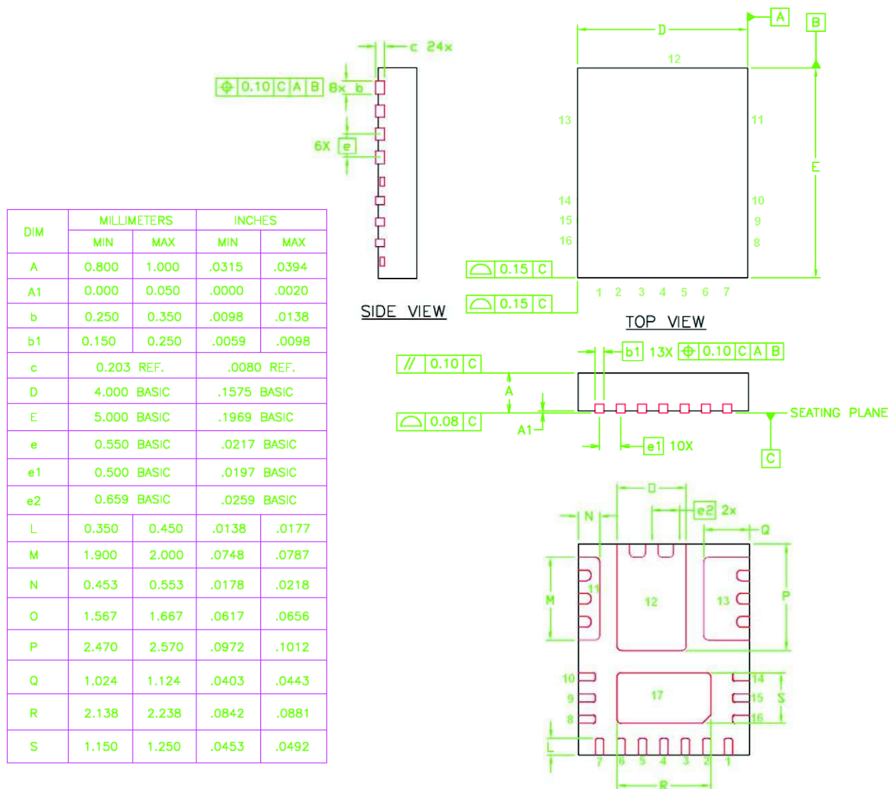
Figure 34: Package Dimensions
