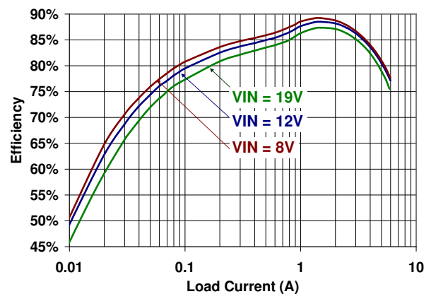
Figure 2: IR3473 Efficiency
