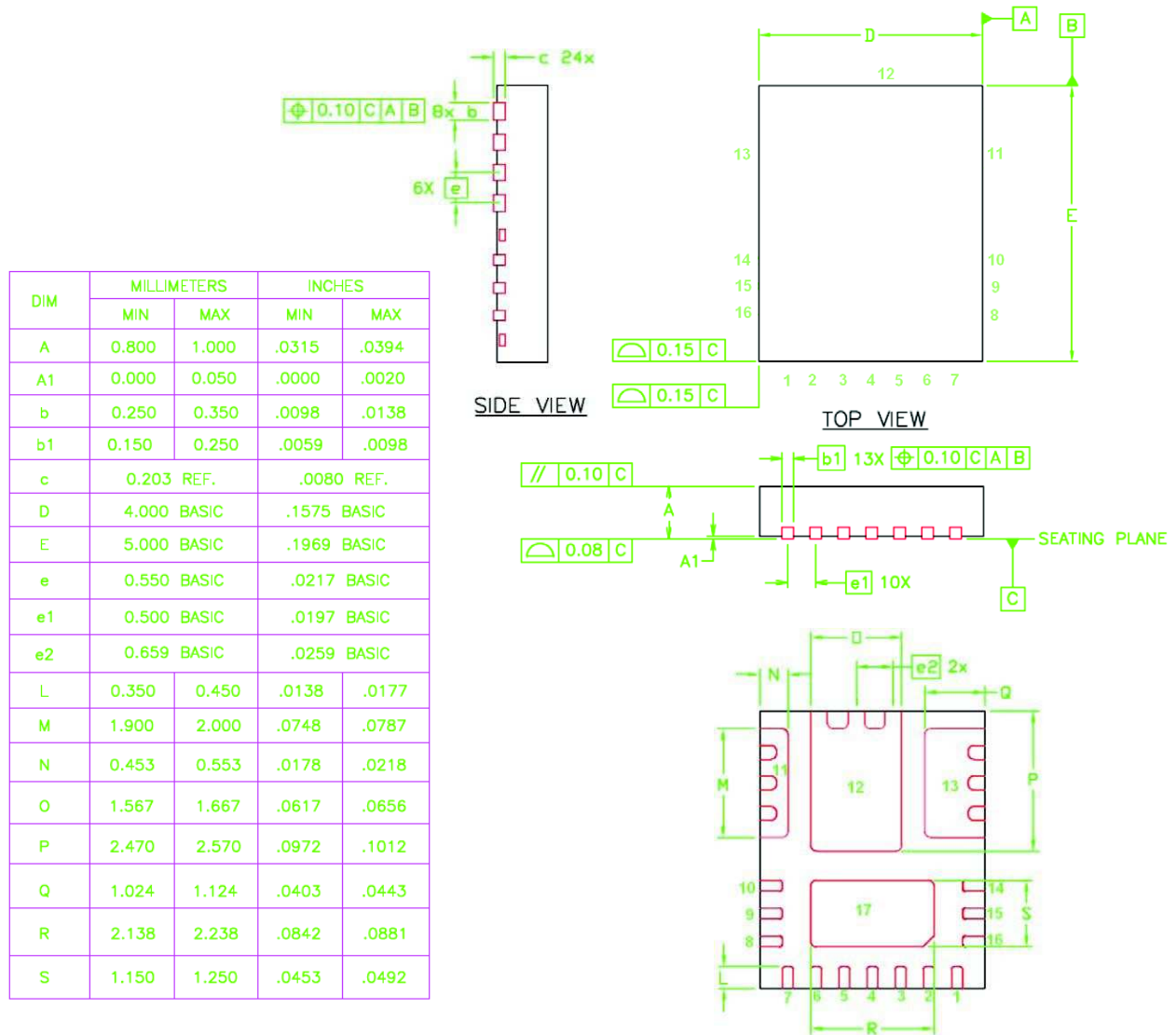
Figure 34: Package Dimensions
