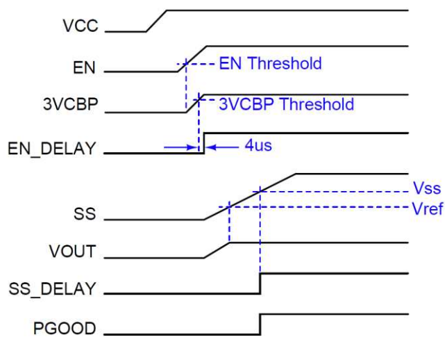
Figure 23: Normal Startup
