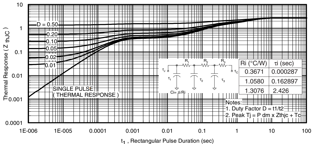
Fig 17. Maximum Effective Transient Thermal Impedance, Junction-to-Case
