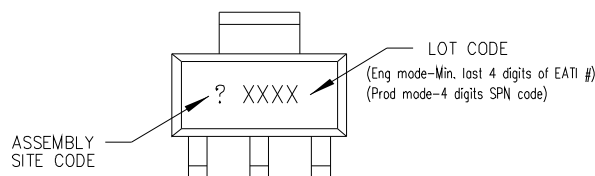
BOTTOM MARKING
