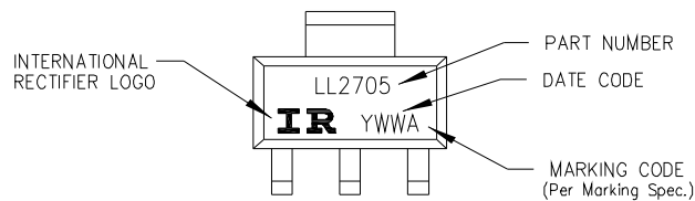
TOP MARKING
