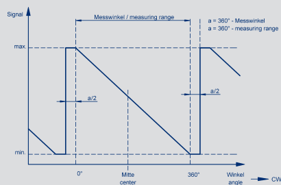
On request: two channel, signal 2 = 0.5 x signal 1
