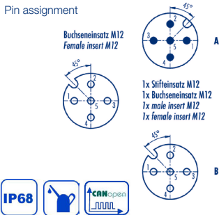
Pin assignment
