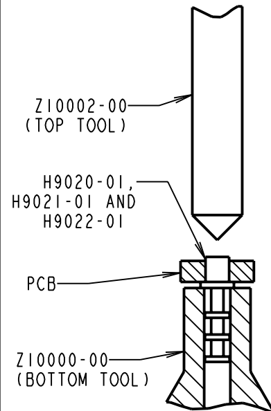
OPERATION DIAGRAM
