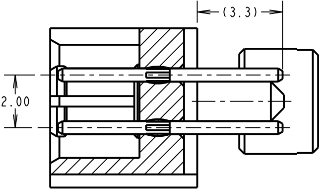
SECTION X-X
