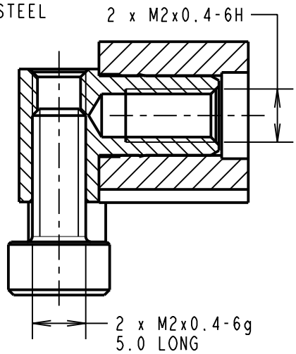
SECTION Y-Y
