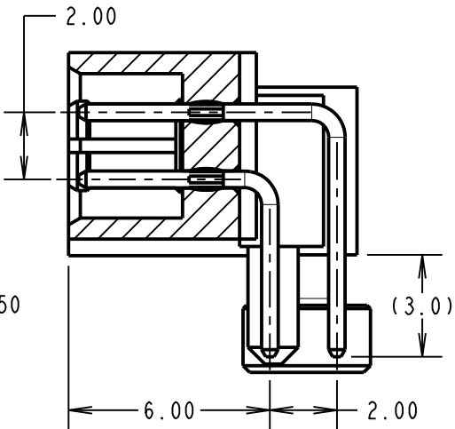
SECTION X-X
