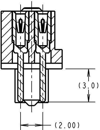
SECTION X-X
