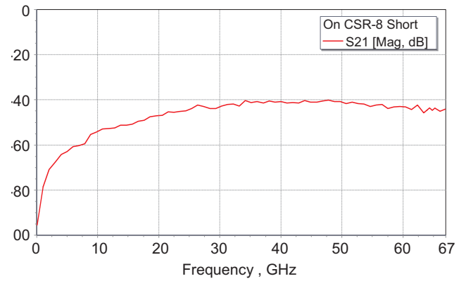
Signal isolation (crosstalk) of two IZI Probes separated by a distance of 150 \mu m.
