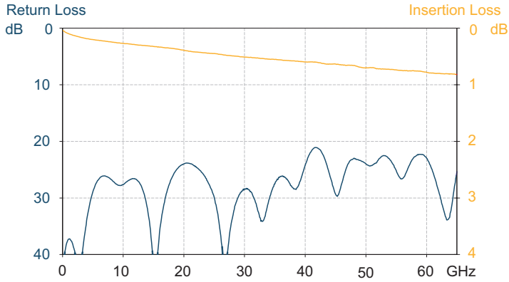
Uncalibrated performance of a IZI Probe 67 V3N GSG 150.
