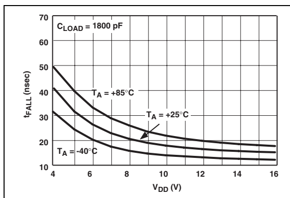
FIGURE 2-10: Fall Time vs. Supply Voltage.
