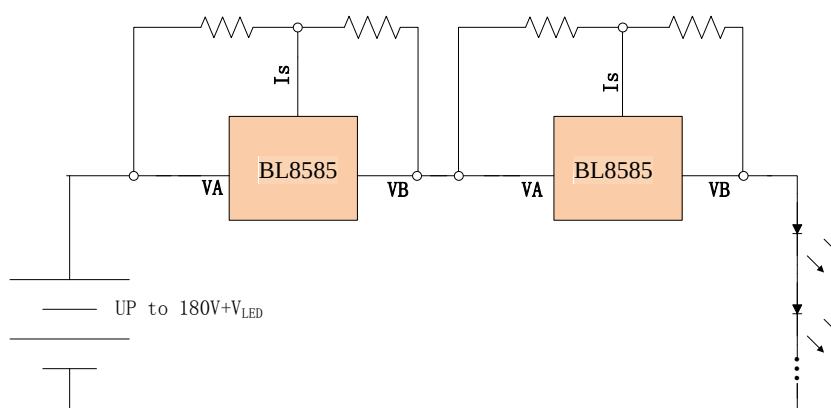
Figure3: For high input voltage use
