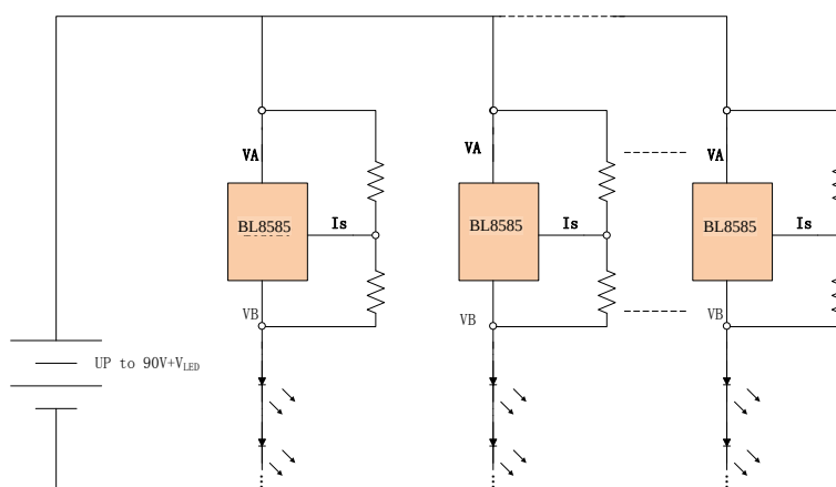
Figure4: For multiple LED strings use
