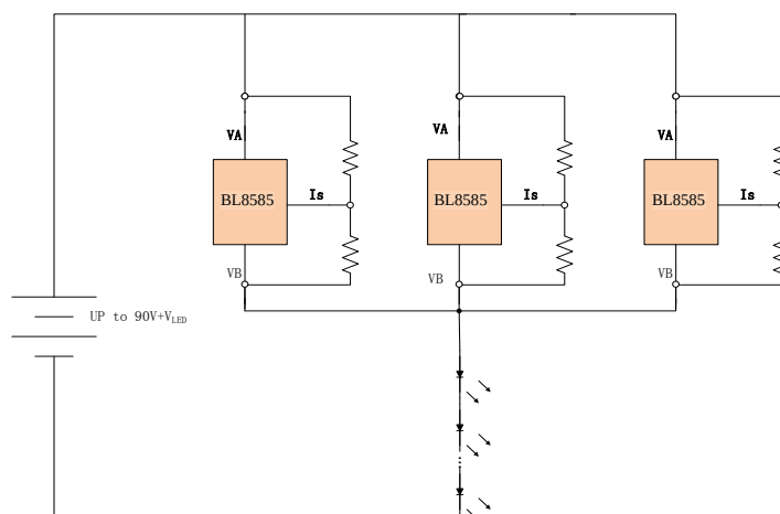
Figure2: For large current use
