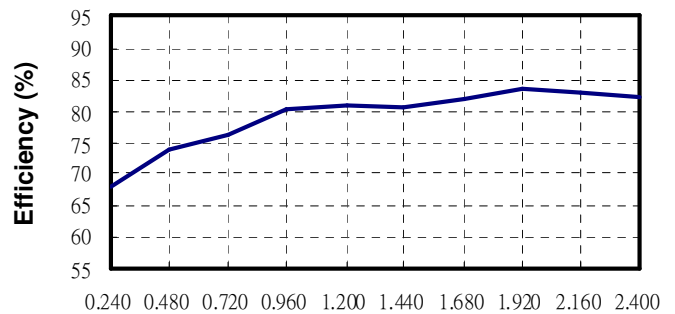
HUB12-48S1H3 Output Current vs. Efficiency
