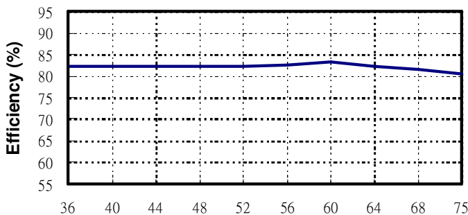
HUB12-48S1H3 Input voltage vs. Efficiency
