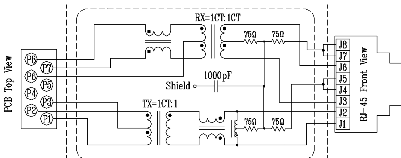
Block Circuit x 1 set in LU1T516 LF
