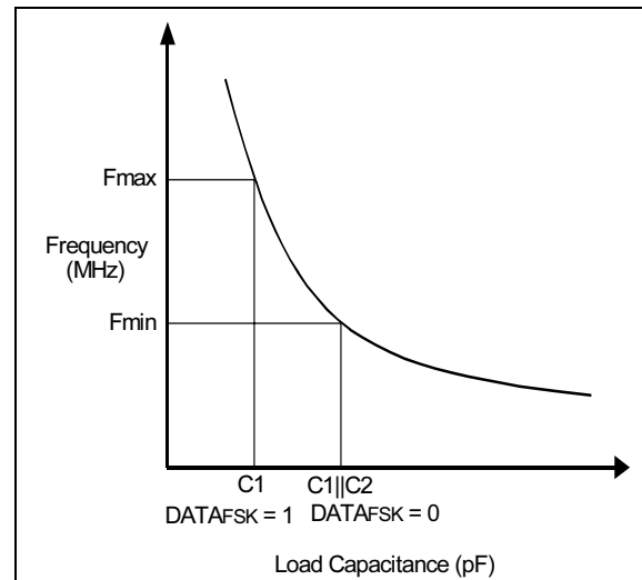
FIGURE 9-4: FREQUENCY PULLING
