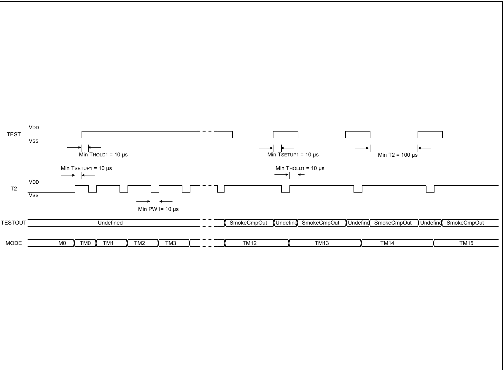
FIGURE 4-5: Timing Diagram for Sensitivity Verification in Mode TM12 ~ TM15.
