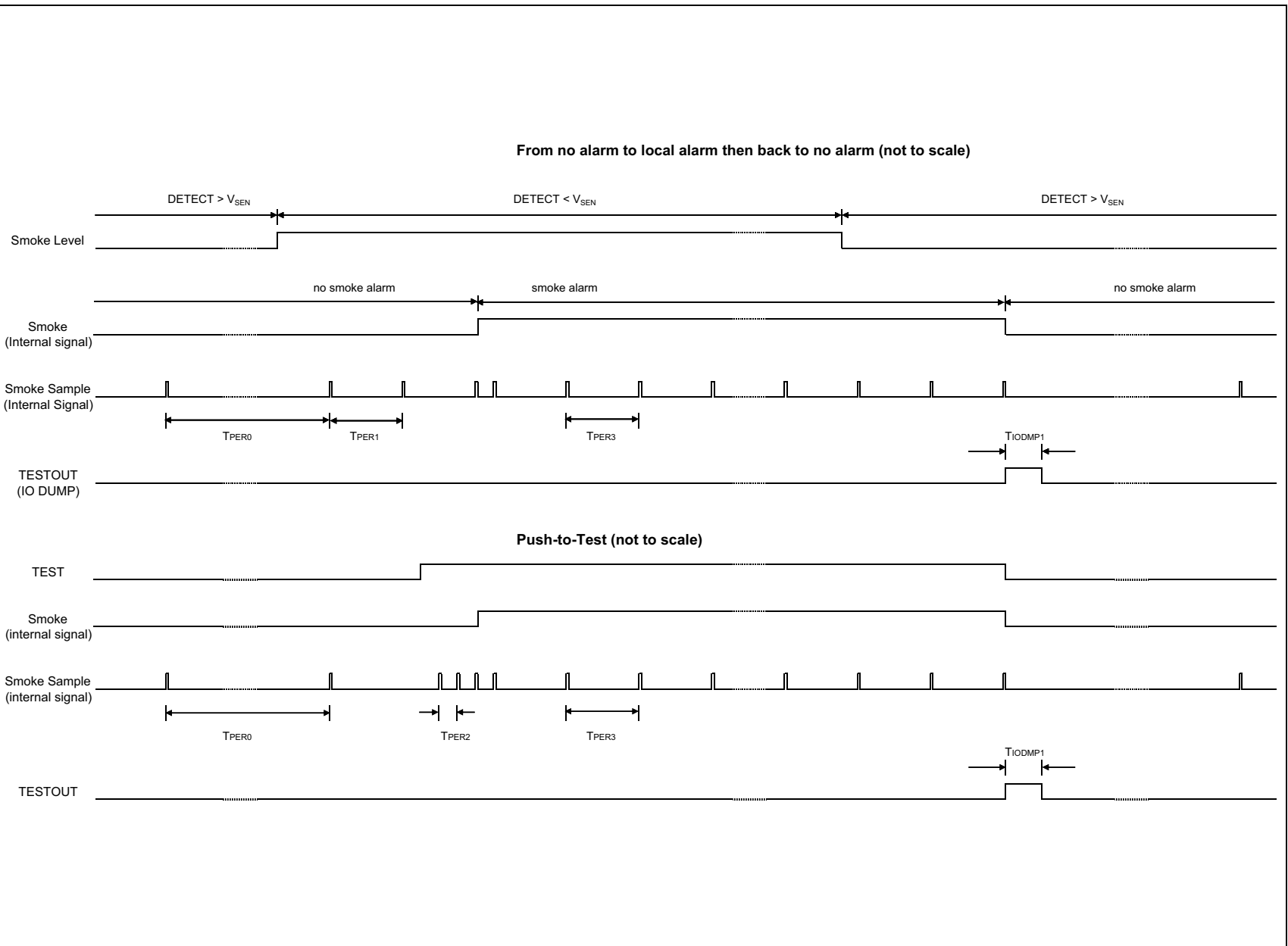
FIGURE 5-3: Timing Diagram – From Standby to Local Smoke and Push-To-Test.
