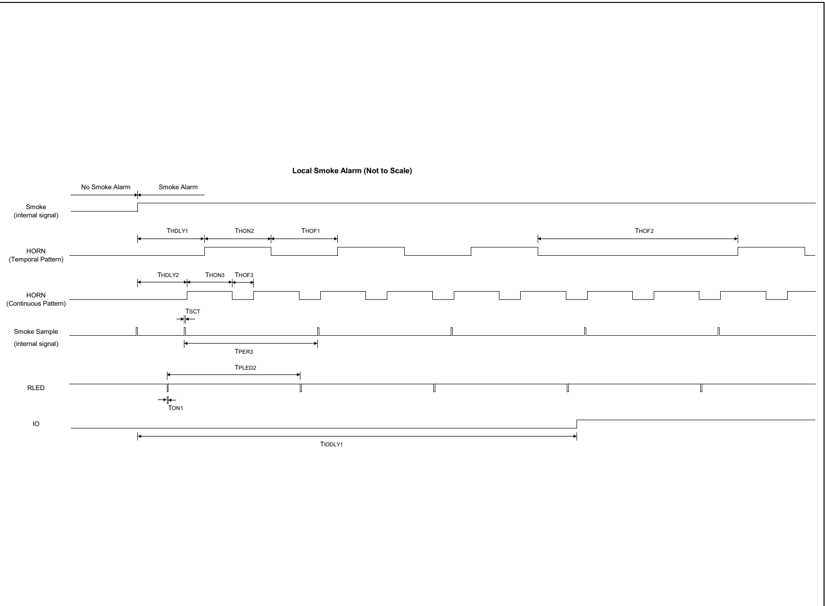
FIGURE 5-4: Timing Diagram – Local Smoke Alarm.
