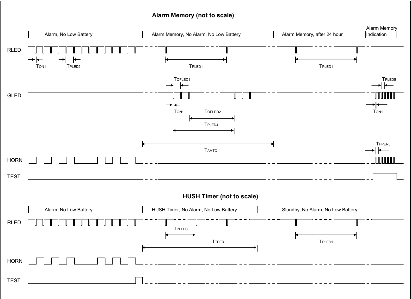
FIGURE 5-6: Timing Diagram – Alarm Memory and HUSH Timer.
