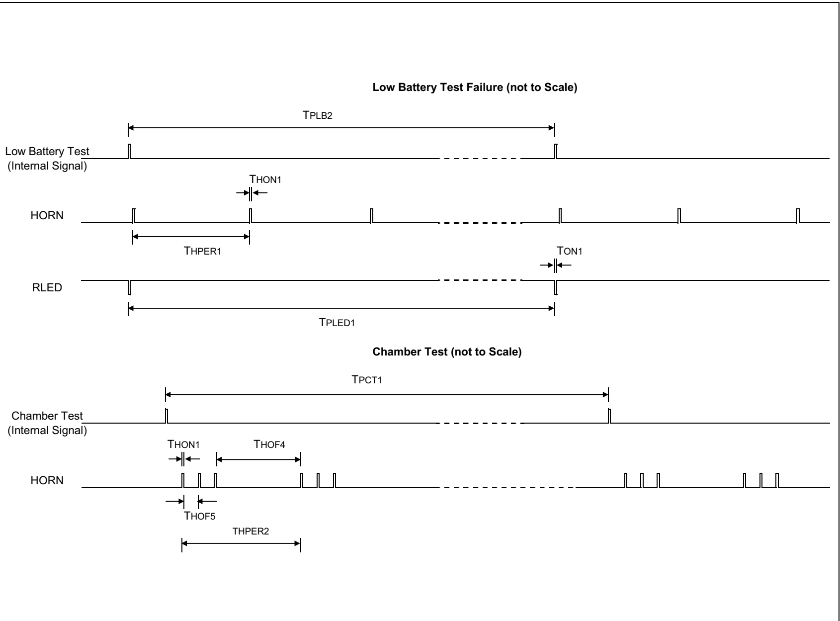
FIGURE 5-2: Timing Diagram – Low Battery Test Failure and Chamber Test Failure.
