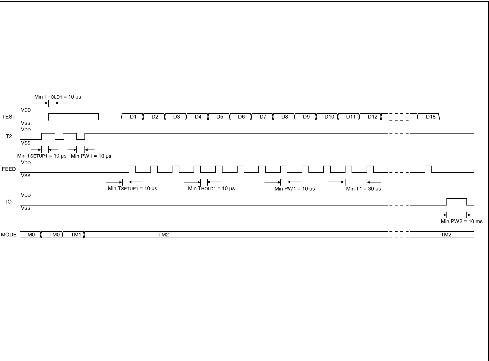
FIGURE 4-4: Timing Diagram for Mode TM2.
