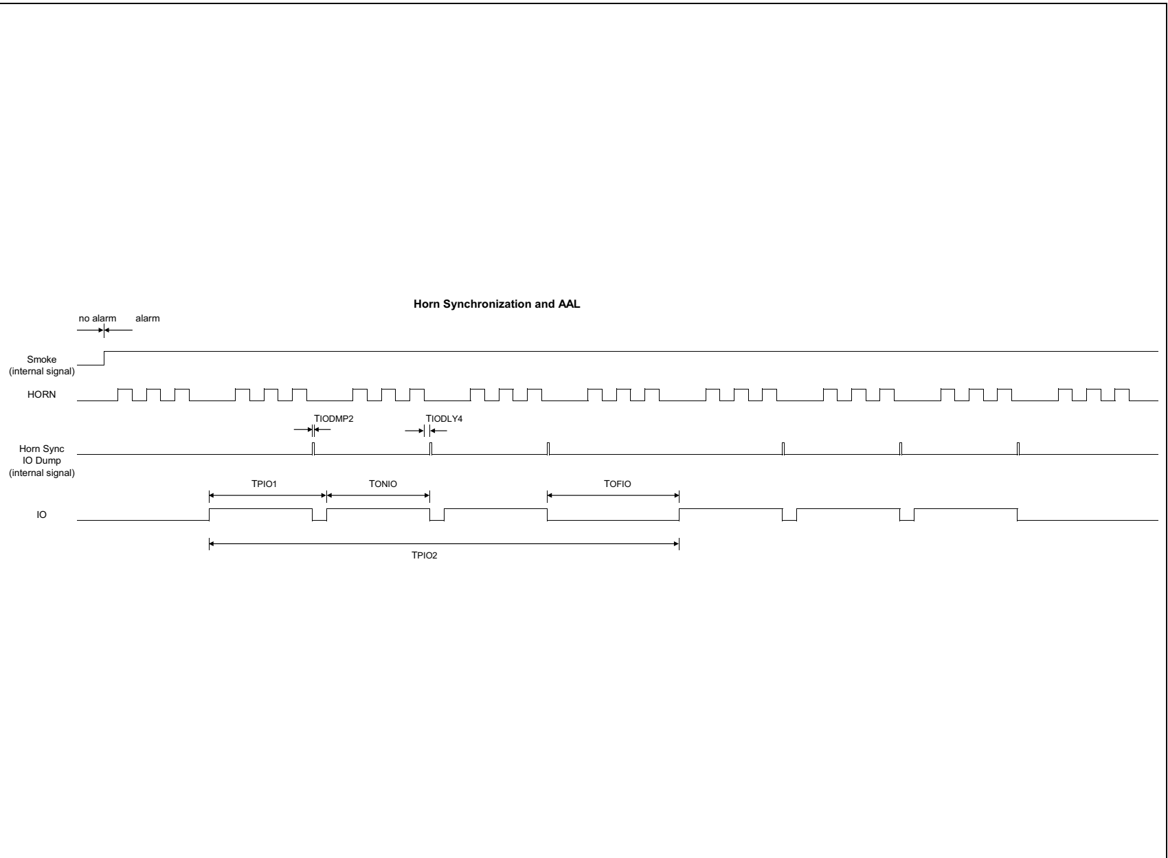
FIGURE 5-8: Timing Diagram – Horn Synchronization and AAL.
