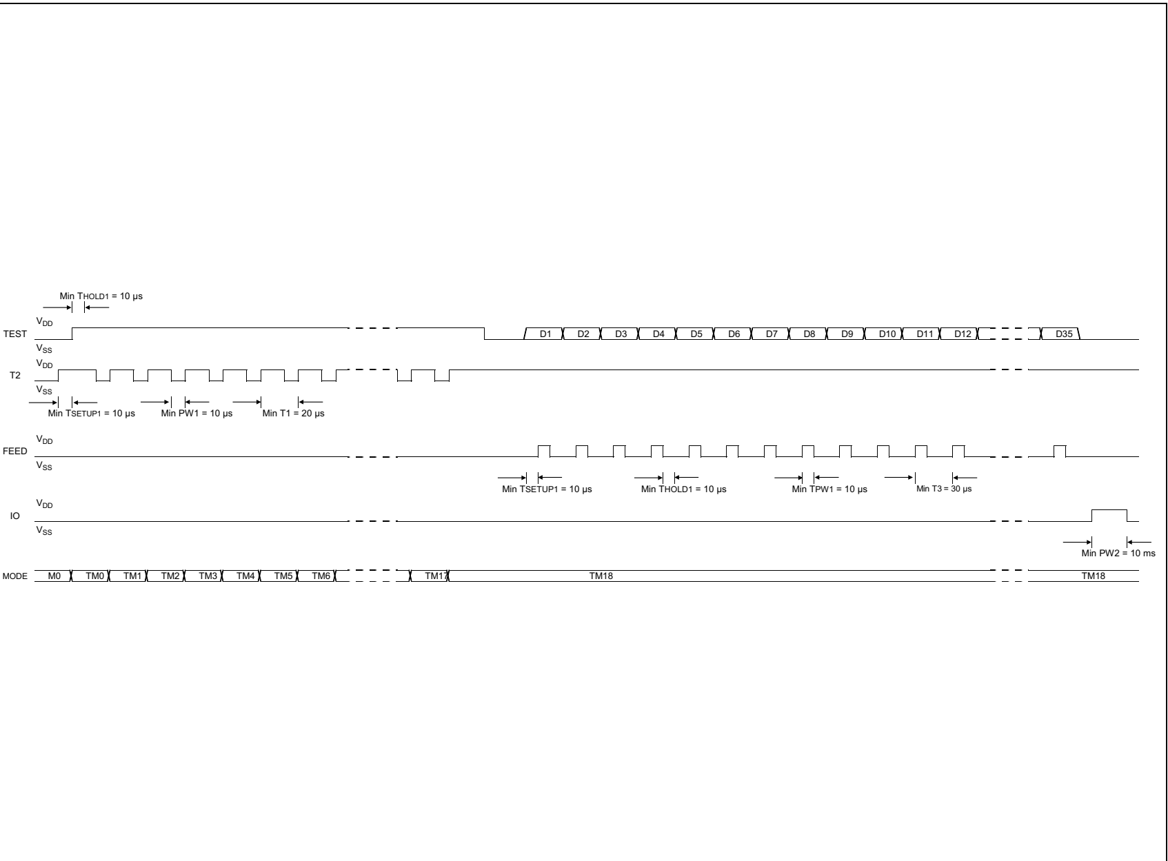
FIGURE 4-6: Timing Diagram for Serial Read/Write Calibration and User Features in Mode TM18.
