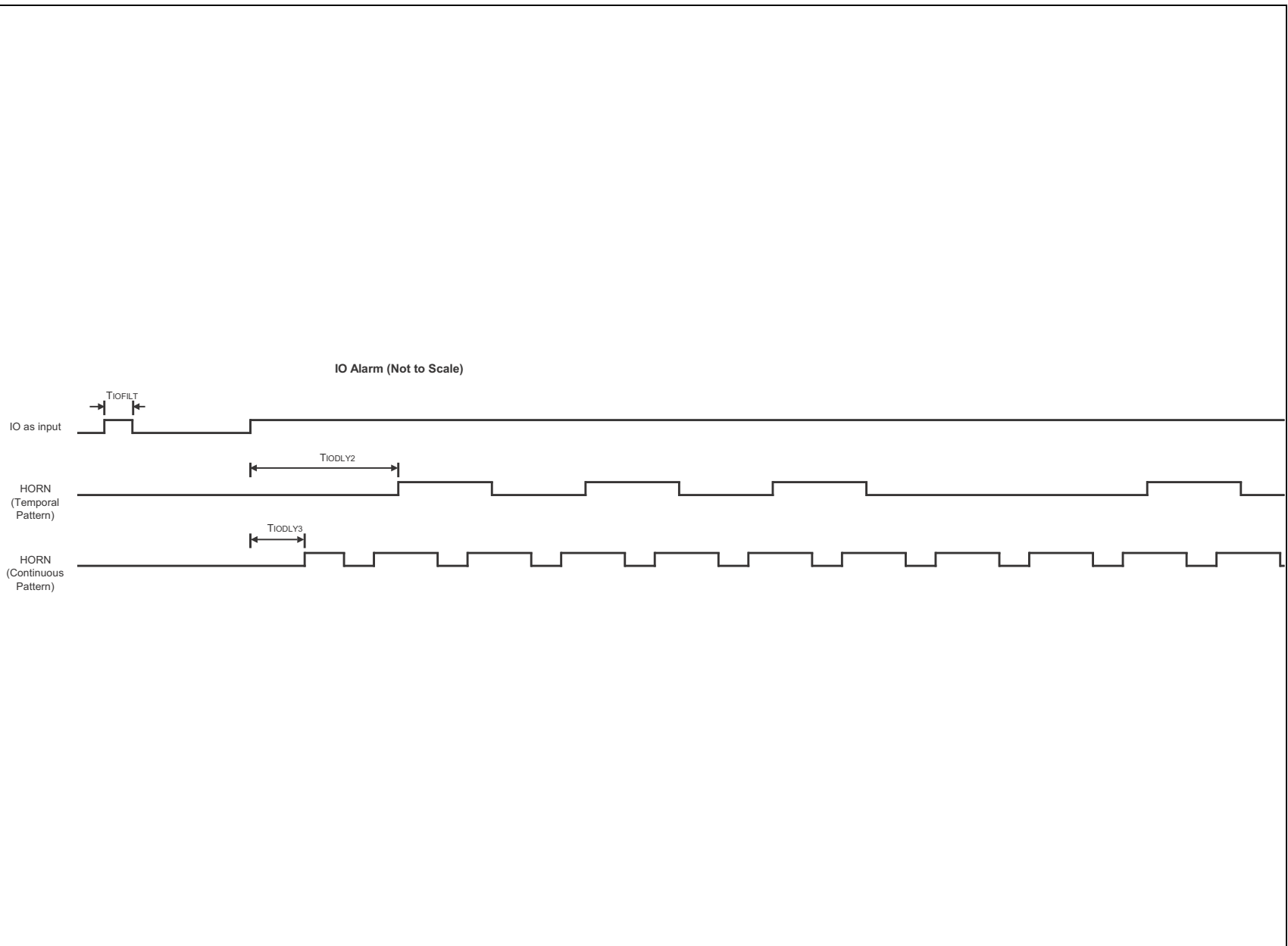
FIGURE 5-5: Timing Diagram – IO Smoke Alarm.
