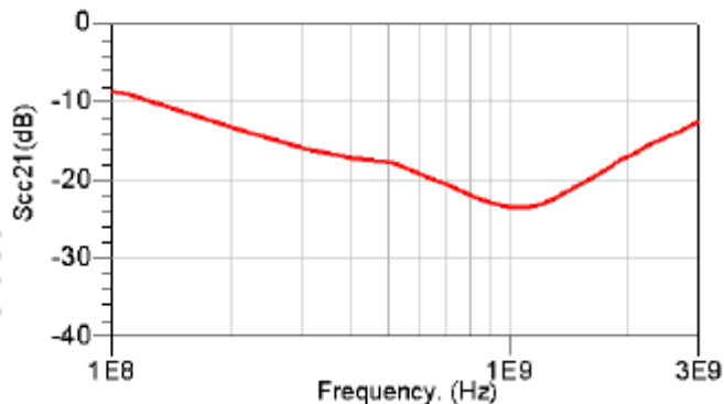
Insertion Loss vs Frequency Characteristic:
