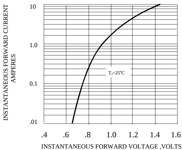
FIG. 3-TYPICAL FORWARD CHARACTERISTICS
