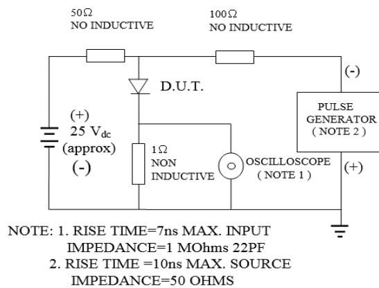
FIG. 1-TEST CIRCUIT DIAGRAM AND REVERSE RECOVERY TIME CHARACTERISTIC
