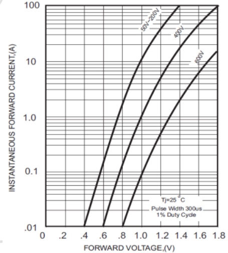
FIG.2-TYPICAL FORWARD CHARACTERISTICS
