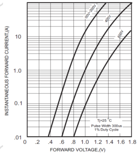
FIG.2-TYPICAL FORWARD CHARACTERISTICS
