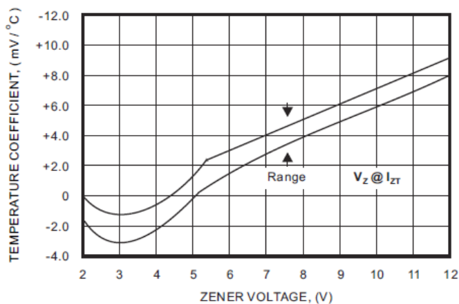
FIG.2A Range for Units to 12 Volts
