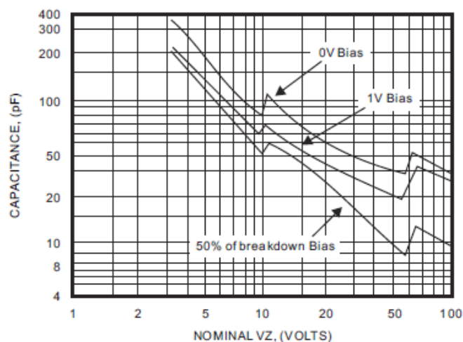
Fig 5. Effect of Zener Current
