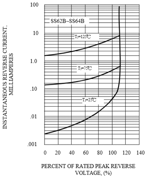
FIG. 3A - TYPICAL REVERSE CHARACTERISTICS
