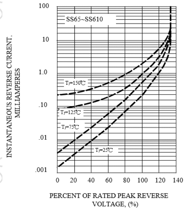
FIG. 3B - TYPICAL REVERSE CHARACTERISTICS
