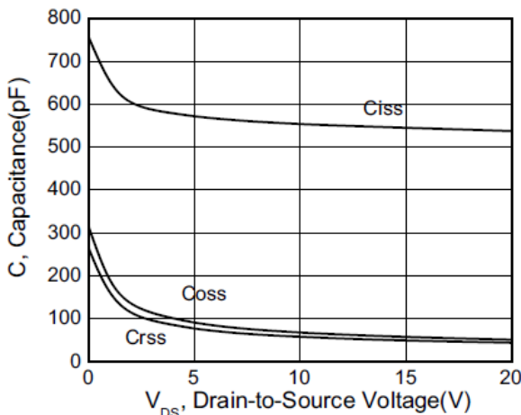
Figure 3. Capacitance
