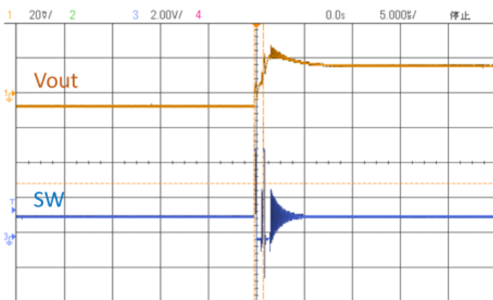
Switching Waveform: VIN=5V, VOUT=1.2V, IOUT=0 mA
