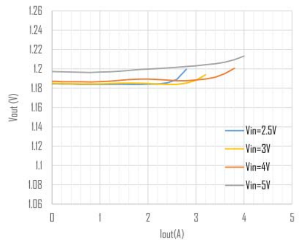
Output Voltage Vs I_{out} , V_{out}=1.2V
