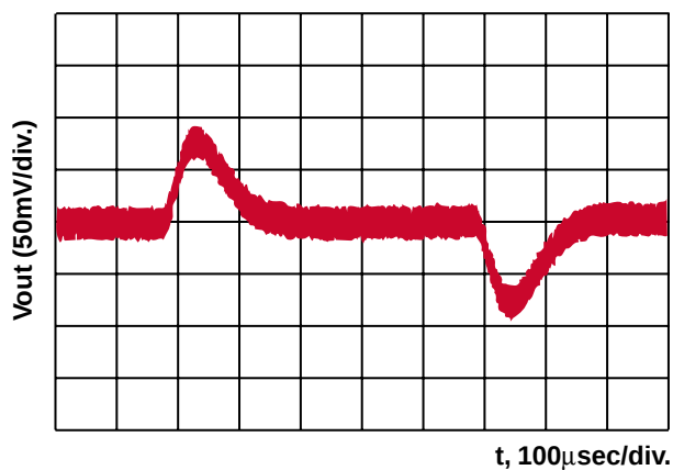
Transient Response
