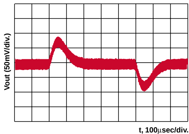
Transient Response
