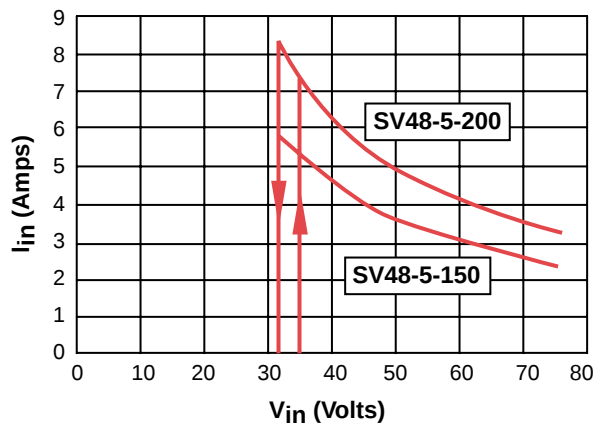
Input Characteristic (room temperature, full load)
