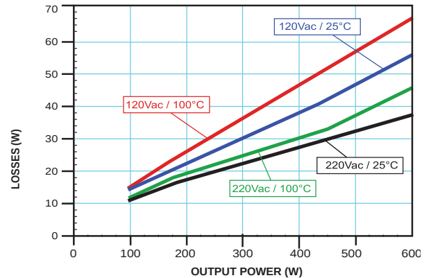
LOSSES CURVE (F=60Hz)
