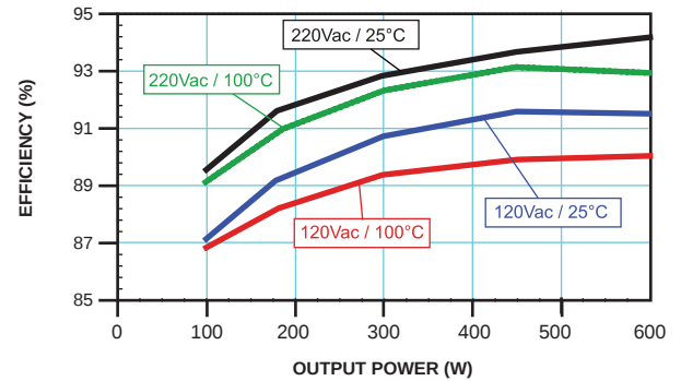
EFFICIENCY CURVE (F=60Hz)
