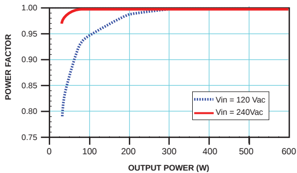
POWER FACTOR CURVE (F=60Hz, Tc = 25 °C)
