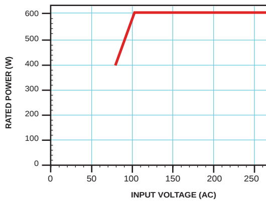
INPUT DE-RATING CURVE
