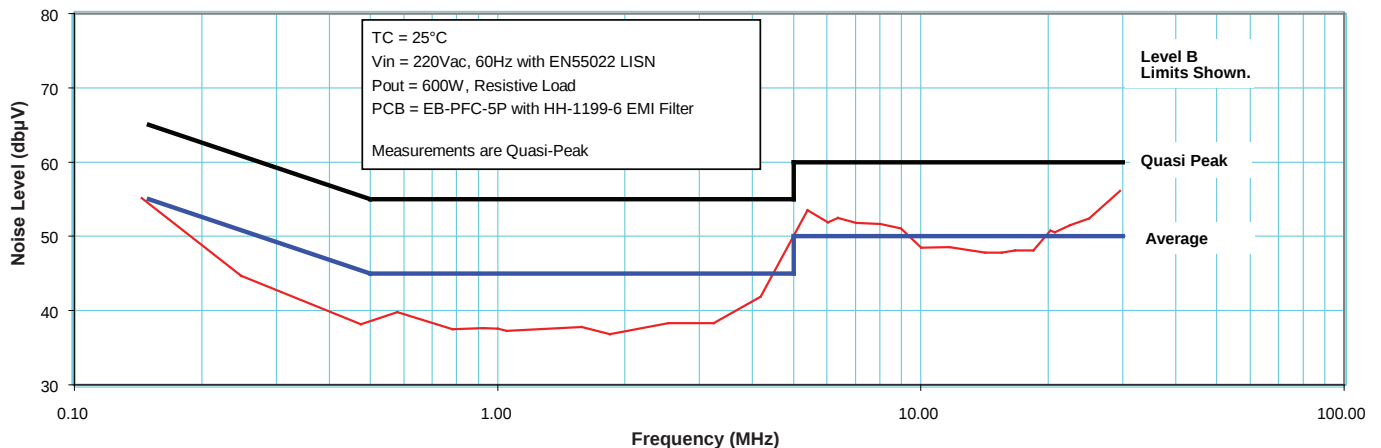
EMI PERFORMANCE - CONDUCTED EMISSIONS
