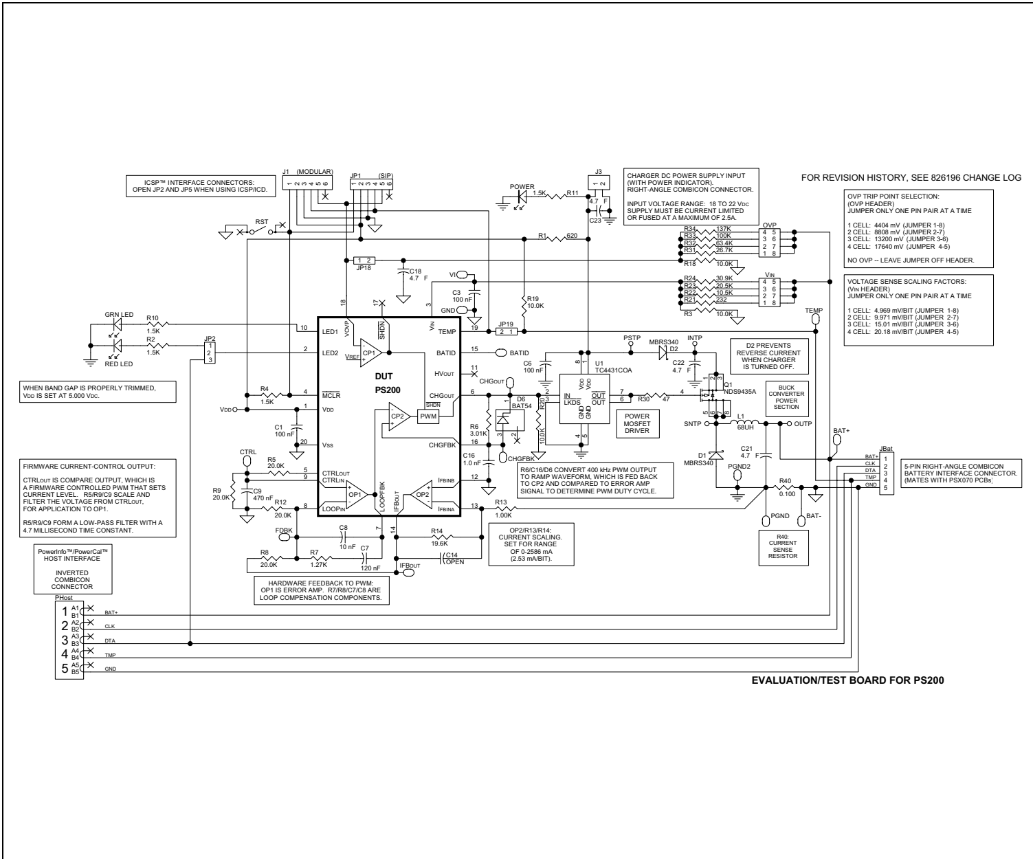
FIGURE 4-1: PS2070 BOARD SCHEMATIC
