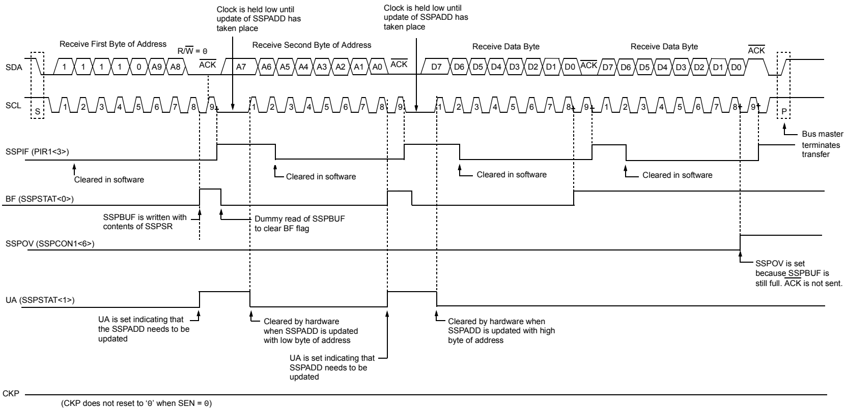
FIGURE 18-11: I 2 C™ SLAVE MODE TIMING WITH SEN = 0 (RECEPTION, 10-BIT ADDRESSING)
