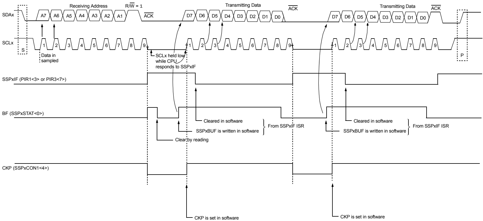
FIGURE 18-10: I 2 C™ SLAVE MODE TIMING (TRANSMISSION, 7-BIT ADDRESSING)
