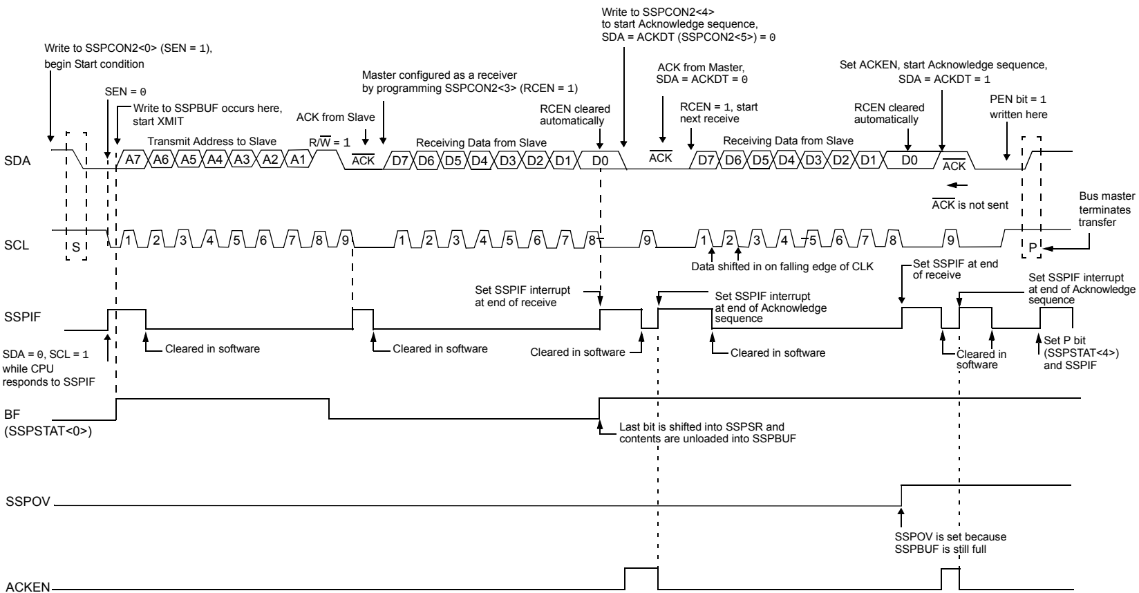
FIGURE 18-24: I 2 C™ MASTER MODE WAVEFORM (RECEPTION, 7-BIT ADDRESSING)
