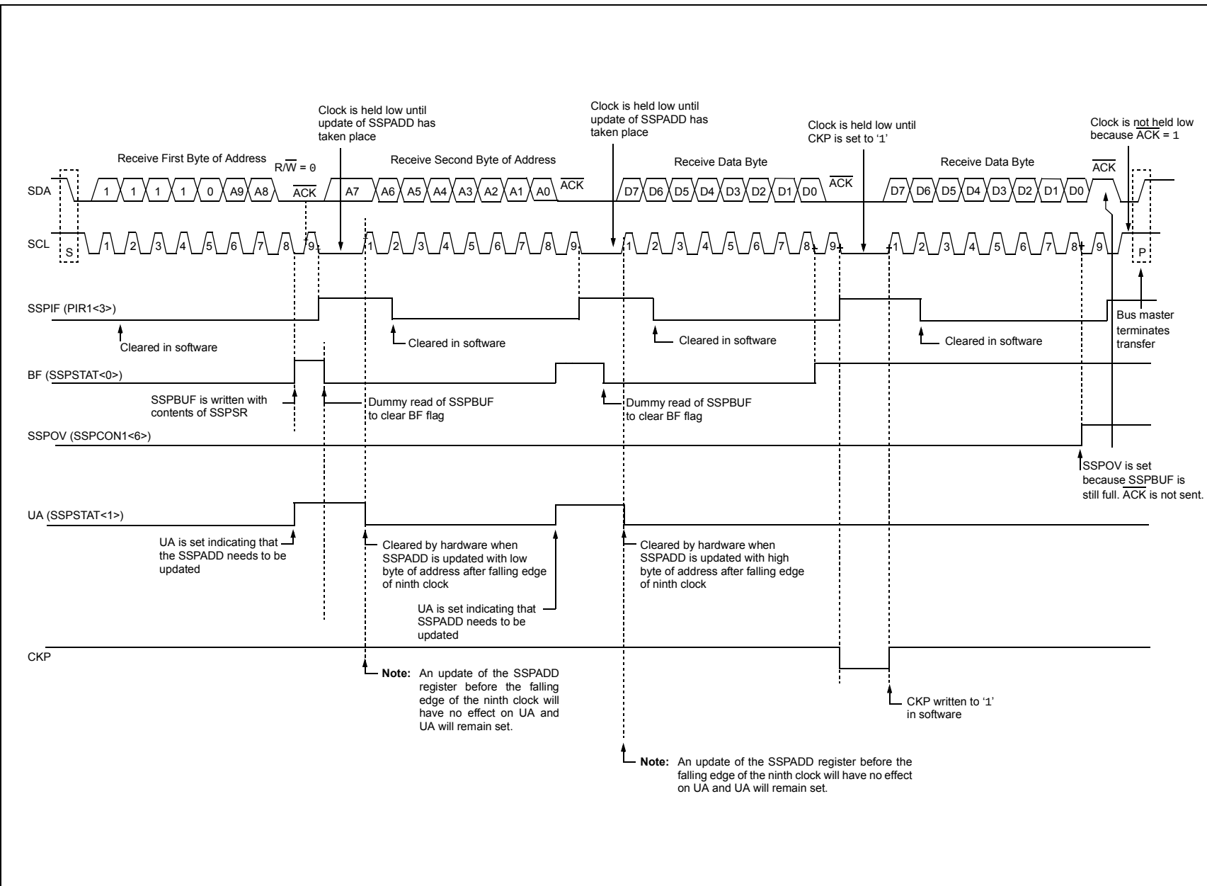
FIGURE 18-16: I 2 C™ SLAVE MODE TIMING WITH SEN = 1 (RECEPTION, 10-BIT ADDRESSING)
