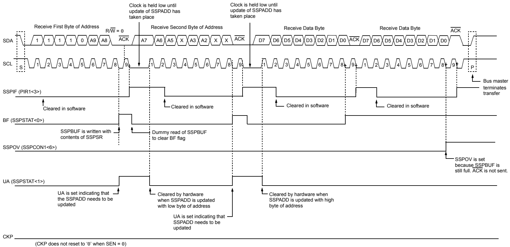
FIGURE 18-12: I 2 C™ SLAVE MODE TIMING WITH SEN = 0 AND ADMSK<5:1> = 010001 (RECEPTION, 10-BIT ADDRESSING)
