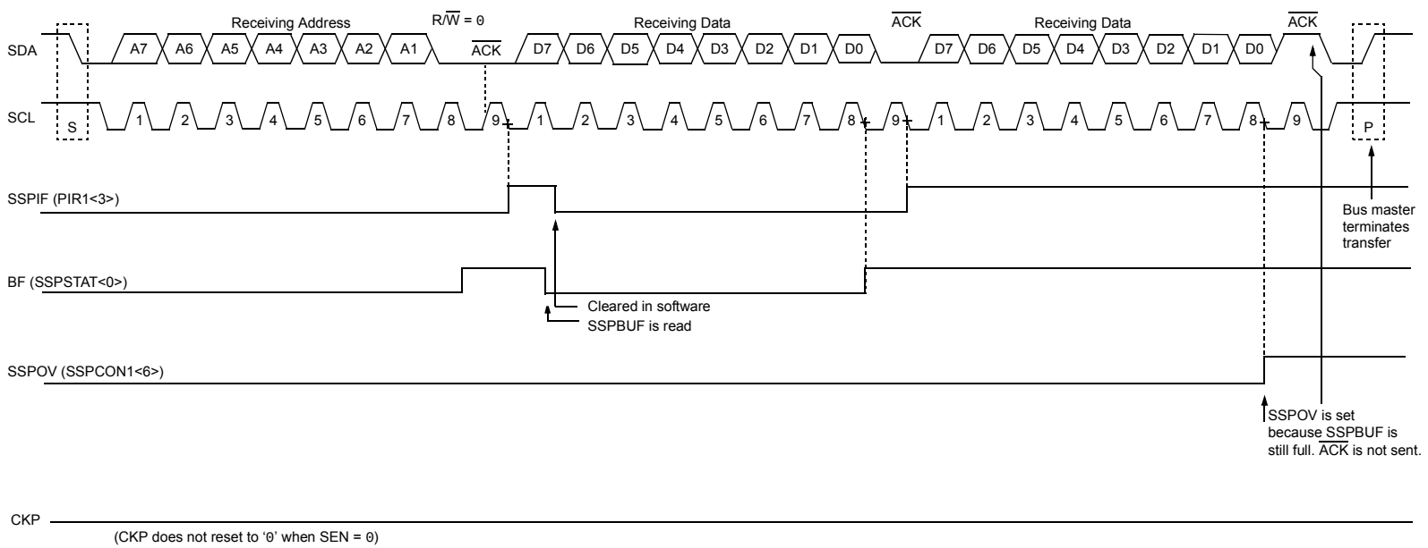
FIGURE 18-8: I 2 C™ SLAVE MODE TIMING WITH SEN = 0 (RECEPTION, 7-BIT ADDRESSING)
