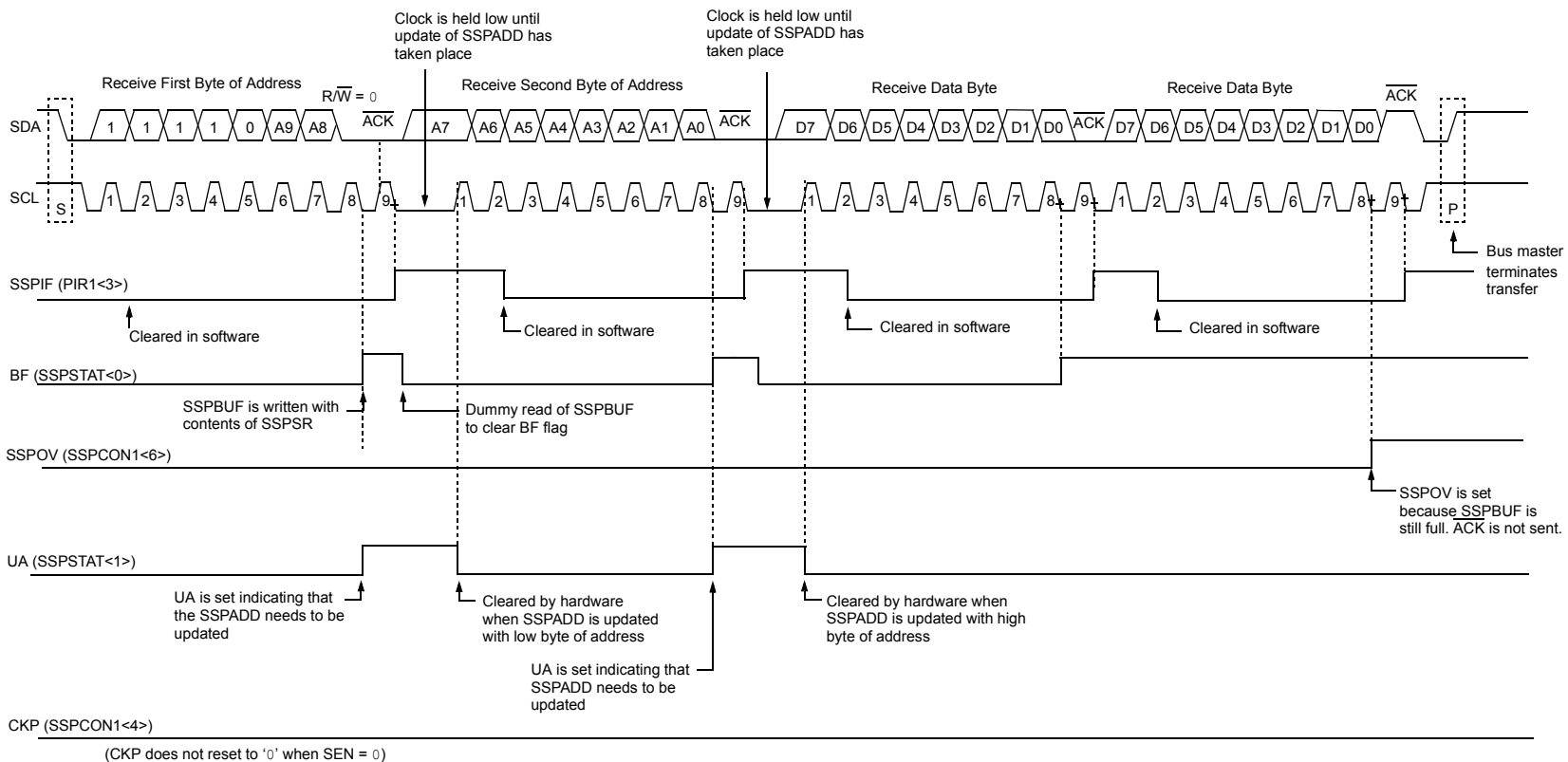
FIGURE 15-10: I 2 C™ SLAVE MODE TIMING WITH SEN = 0 (RECEPTION, 10-BIT ADDRESS)
