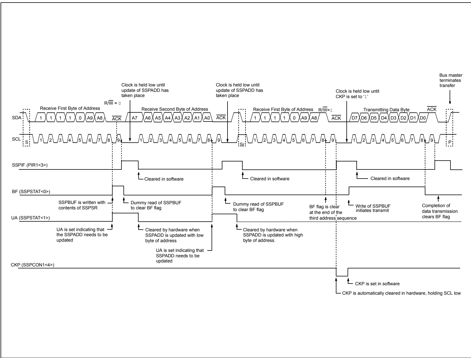
FIGURE 15-11: I 2 C™ SLAVE MODE TIMING (TRANSMISSION, 10-BIT ADDRESS)
