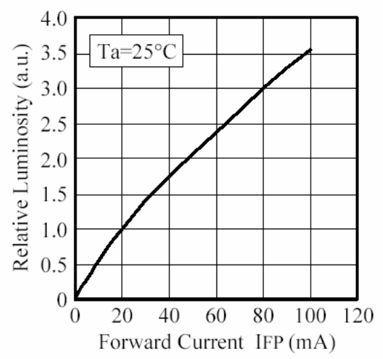
■ Forward Current vs. Relative Luminosity
