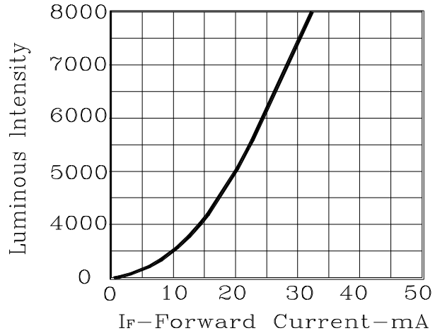
■ Ta= 25°C Luminous Intensity VS. Forward Current (Mcd)
