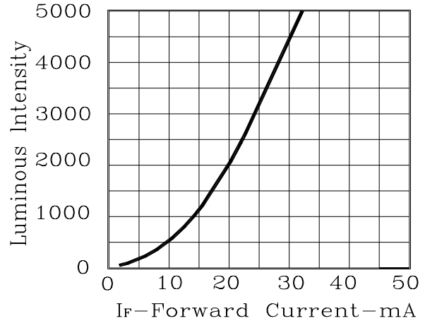
■ T_J = 25^\circ\text{C} Luminous Intensity VS. Forward Current
