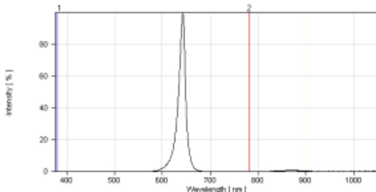
Fig.1 Super Red Relative Intensity vs. Wavelength
