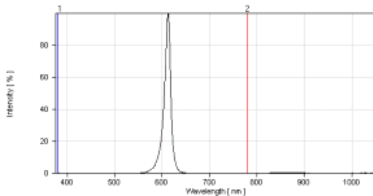
Fig.2 Super Amber Relative Intensity vs. Wavelength
