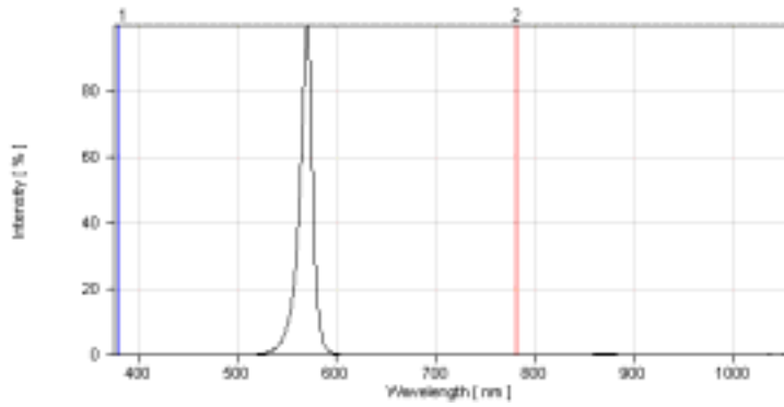
Fig.1 Super Green Relative Intensity vs. Wavelength
